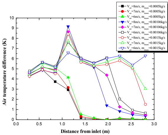
Fig. 10 Air temperature difference distributions of finned tube experiments
