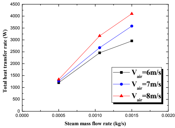
Fig. 9 Total heat transfer rates of finned tube experiments along with steam mass flow rate and air velocity
