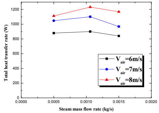
Fig. 5 Total heat transfer rate along with steam mass flow rate and air velocity
