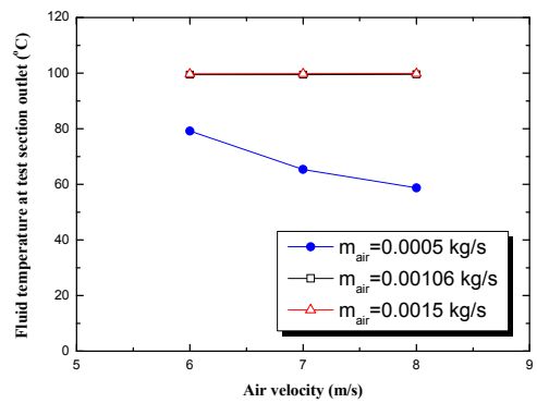
Fig. 6 Outlet fluid temperature along with steam mass flow rate and air velocity
