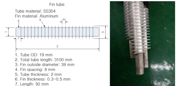
Fig. 3 Specifications and picture of finned tube for experiments
