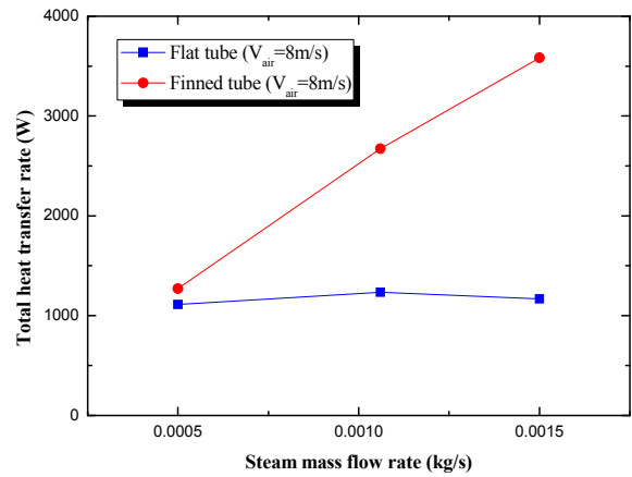
Fig. 12 Comparison of total heat transfer rate between flat tube and finned tube
