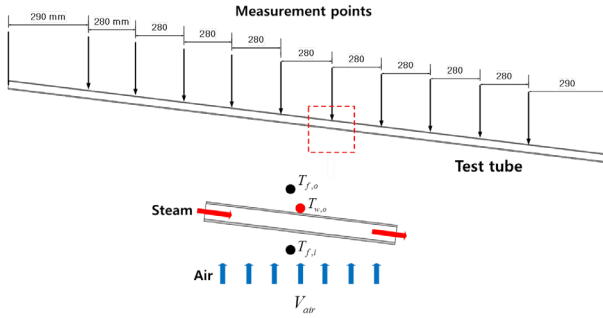
Fig. 4 Measurement points of heat transfer parameters on test section
