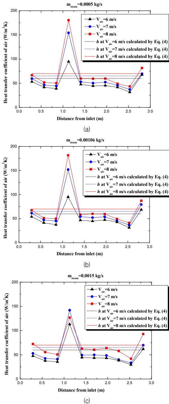
Fig. 7 Air-side heat transfer coefficient distributions with air velocity; (a) \dot{m}_{steam} = 0.0005 kg/s, (b) \dot{m}_{steam} = 0.00106 kg/s, (c) \dot{m}_{steam} = 0.0015 kg/s
