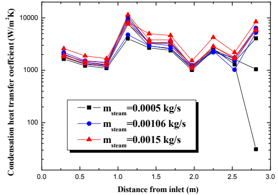
Fig. 8 Condensation heat transfer coefficient distributions along with steam mass flow rates
