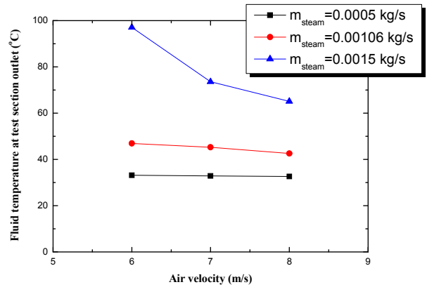
Fig. 11 Outlet fluid temperature of finned tube experiments along with steam mass flow rate and air velocity
