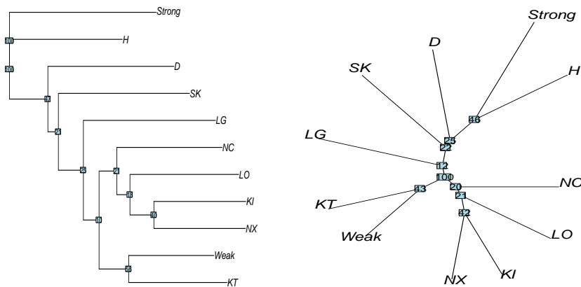
Figure 3.2 Rooted/ unrooted tree diagrams
