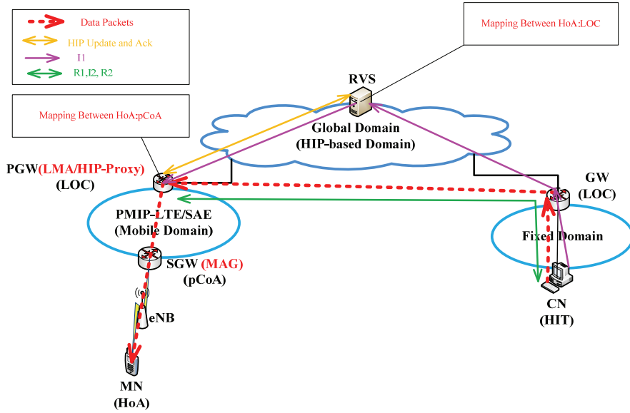
Fig. 4. Network model of HIP-PMIP-LTE/SAE architecture.
