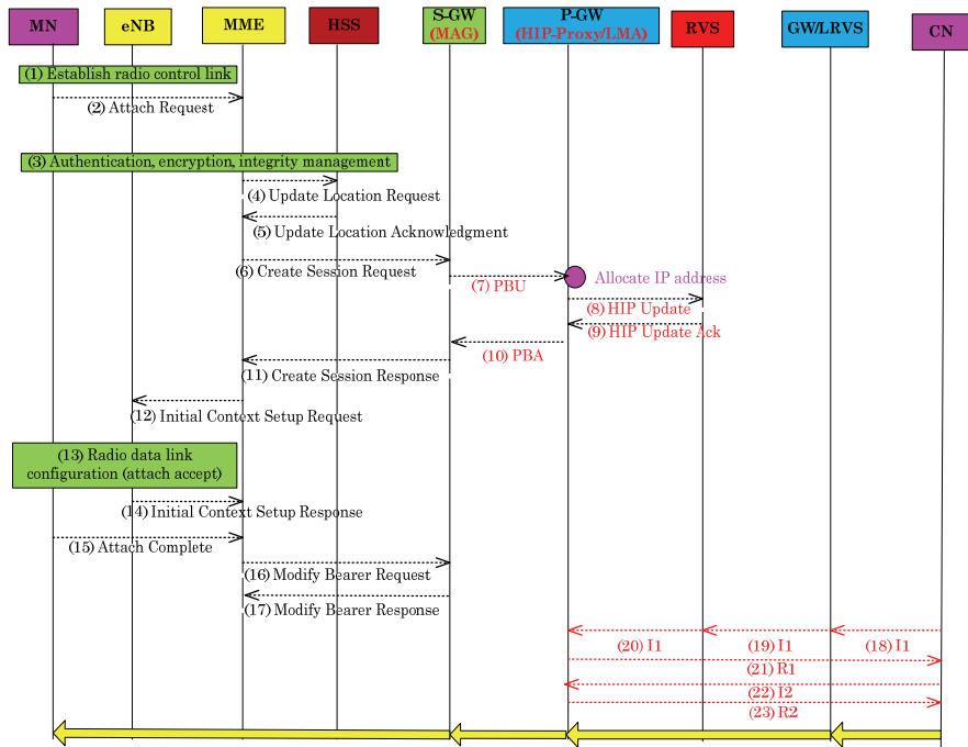
Fig. 5. Binding update and data delivery in HIP-PMIP-LTE/SAE.
