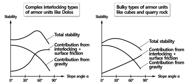
Fig. 2. Influence of slope angle on the stabilizing effects of gravitational force, interlocking and surface friction (after Price 1979).
