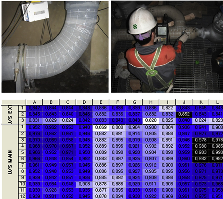
Fig. 1 – Wall thickness measurement and evaluation examples for managing secondary system pipe wall thinning at nuclear power plants.
