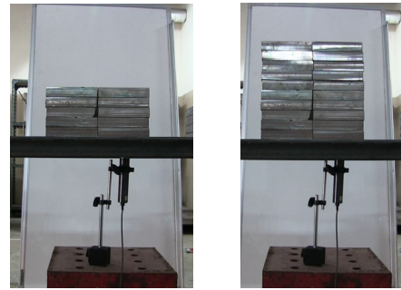
(a) The 100kgf loading (b) The 200kgf loading
