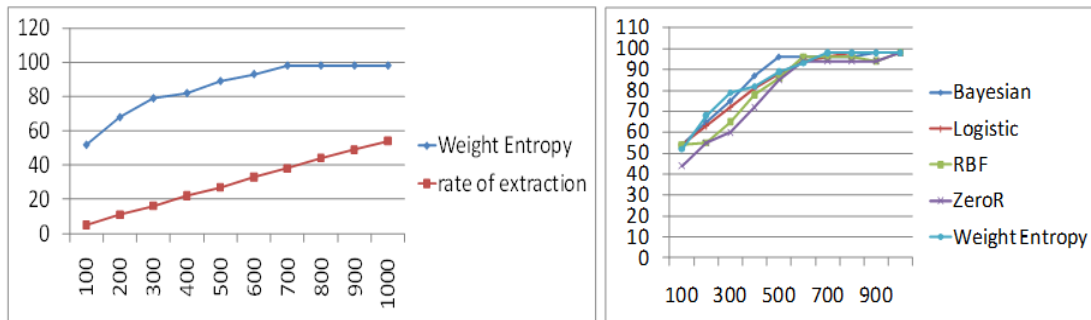
Fig. 4. Comparative results of weight entropy with general mining algorithms
