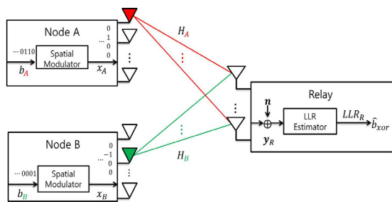
Fig. 2 Transmission/reception procedure of SM-PNC to separate decoding in 1st time slot
