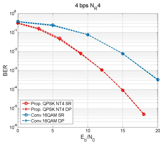
Fig. 10 E_b/N_0 performance of SM-PNC 4bps data rate to 4 relay node antennas (4 transmit antennas, QPSK).
