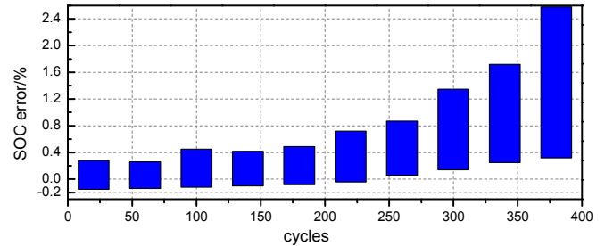
Fig. 20. SOC estimation error margins vs. cycles, 30^{\circ}\text{C} .
