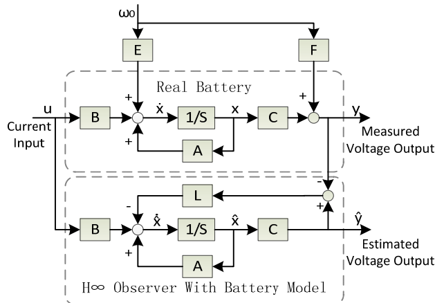
Fig. 16. Schematic diagram of H \infty -based state observer.
