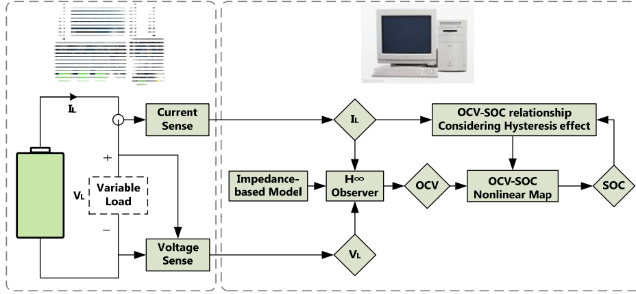
Fig. 9. Schematic illustration of the proposed SOC estimation methodology.
