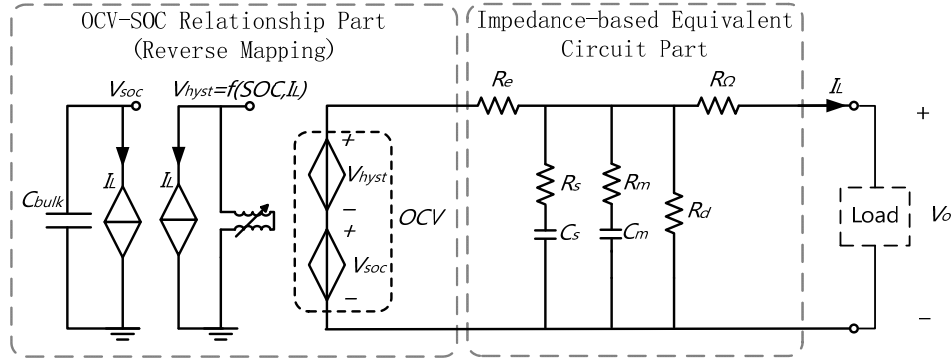
Fig. 12. The combined model of the investigated battery, incorporating equivalent circuit part and OCV-SOC relationship part.
