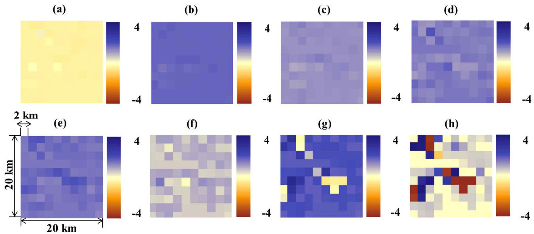
Fig. 9. Monthly soil moisture deficit index (SMDI) at Chungmi-cheon site 1 in 1990; (a-h) March to October.
