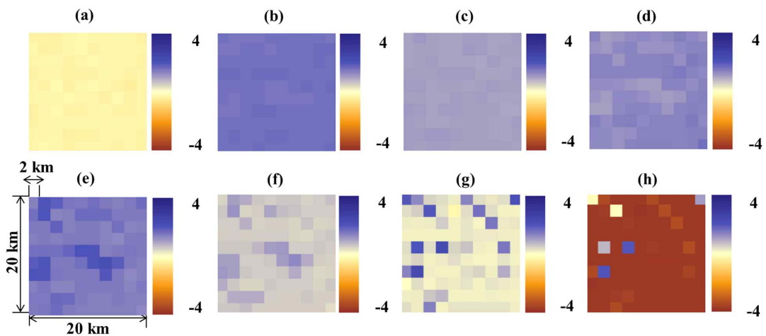
Fig. 11. Monthly soil moisture deficit index (SMDI) at Chungmi-cheon site 2 in 1990; (a-h) March to October.
