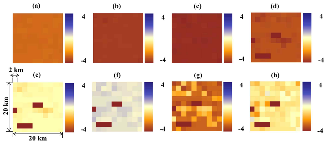
Fig. 12. Monthly soil moisture deficit index (SMDI) at Chungmi-cheon site 2 in 2001; (a-h) March to October.
