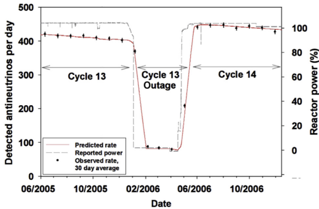
Fig. 4 – Monthly neutrino rates observed by the SONGS detector. It shows the evolution due to changes in the fissile content from burnup. Taken from Fig. 2 in Ref. [24]. It shows the possibility to monitor the reactor fuel contents by measuring the neutrino rates. SONGS, San Onofre Nuclear Generating Station.
