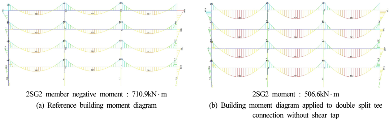
Fig. 6. Comparison of Negative Moment Values
