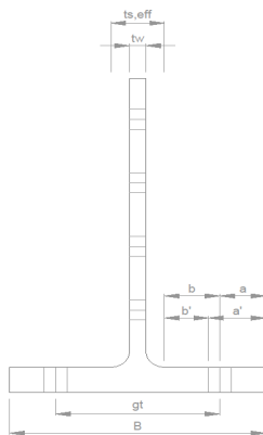
(a) Geometry of T-section flanges
