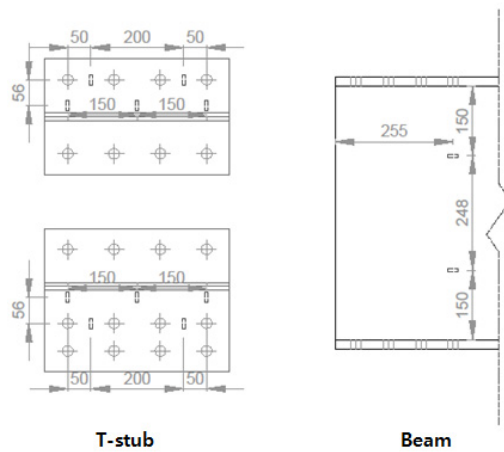
(a) Positions of strain gauges attached
