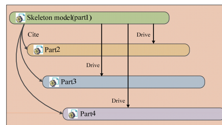
Fig. 3. Design driven by skeleton model
