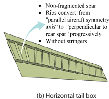
(b) Horizontal tail box
