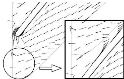
(a) Baseline impeller (9.031 kg/s)
