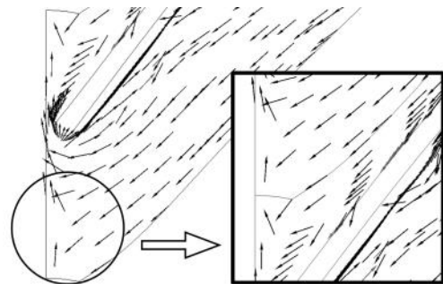
(b) Modified impeller (8.264 kg/s)
