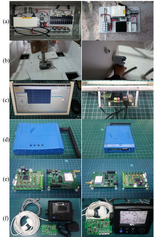
Figure 7: Image of individual components used for eco-environmental leisure boat for this study ;
