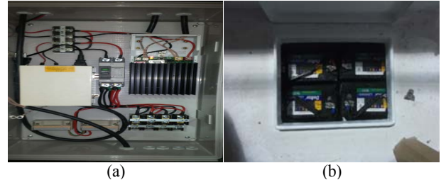
Figure 15: The view of charging inverter component (a), battery for supplying electro-motive force (b)
