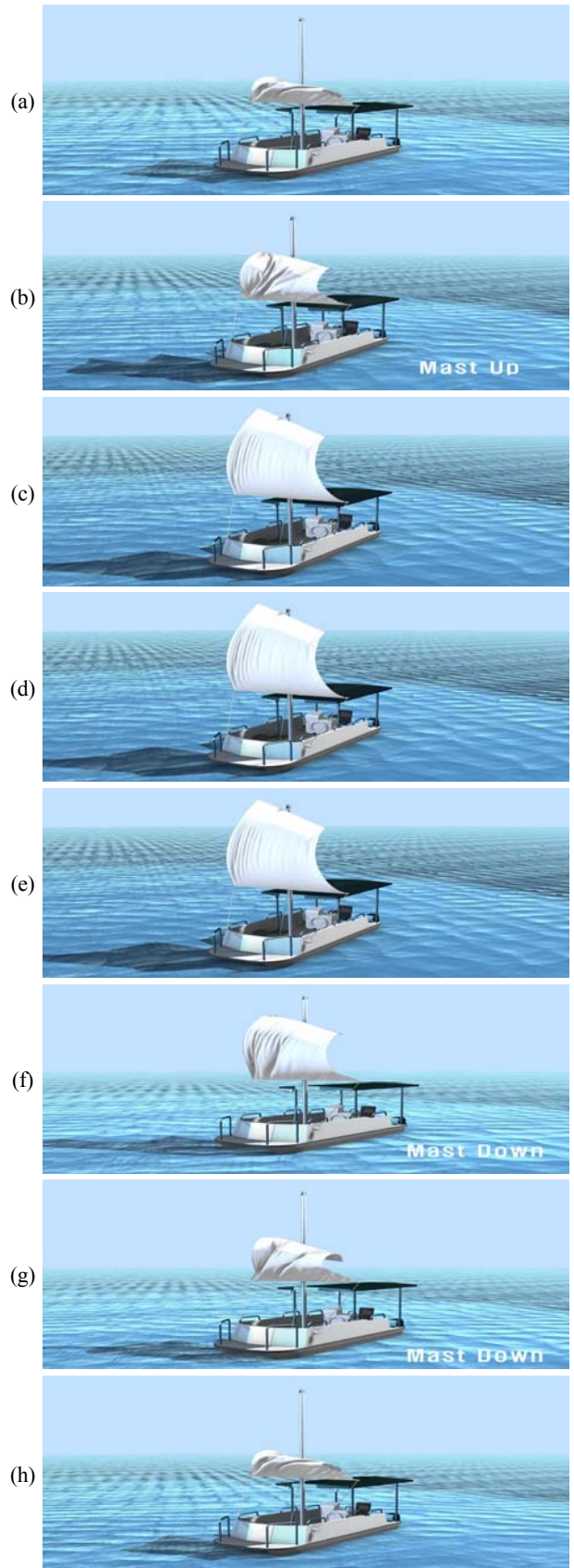
Figure 19: The simulation view of sail up/down system during actual operation; (a) 10%, (b) 50%, (c) 80%, (d) 100% (as sail-up operation state), (e) 10%, (f) 30%, (g) 50%, (h) 100% (as sail-down operation state)
