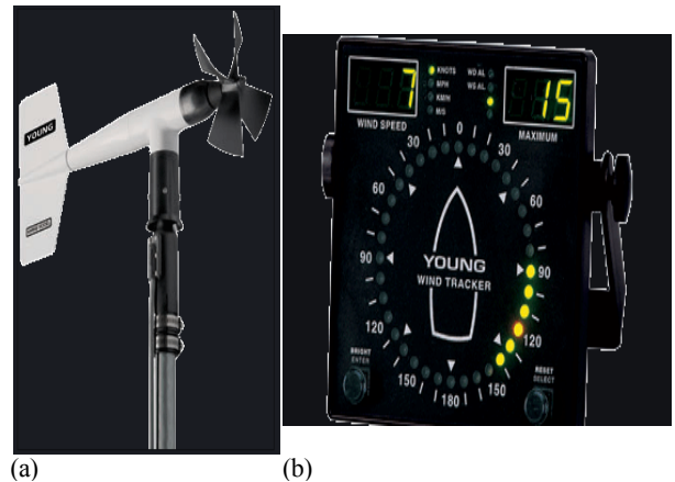
Figure 13: The view of calibration instrument for measuring wind direction and speed; (a) view of instrument, (b) digital type of indicator for wind direction and speed
