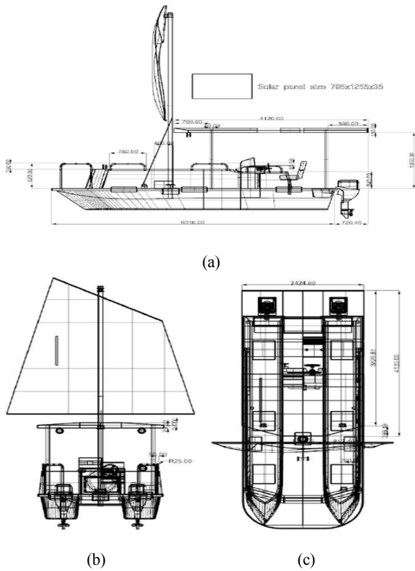
Figure 3: Drawing image with respect to eco-environmental leisure boat with a photovoltaic hybrid generating system ; (a) elevation, (b) section and (c) plan
