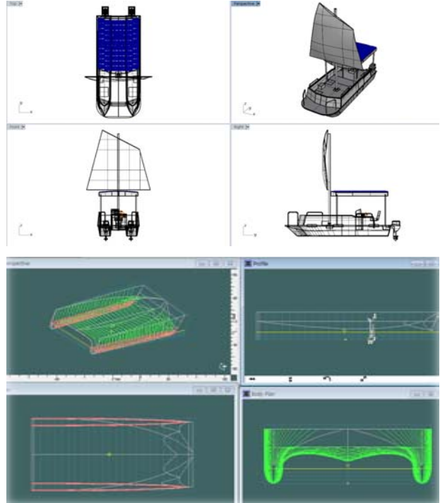
Figure 5: 3D-Modelling image as to the prototype with a hybrid generating system (wind + solar energy)
