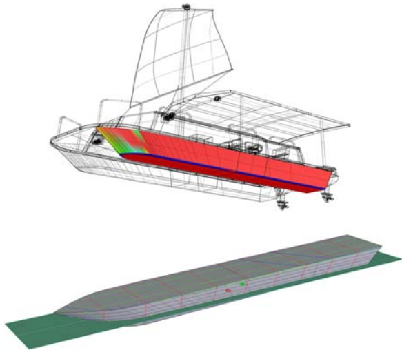
Figure 4: Several schematic modelling image for structural analysis as to the prototype with a photovoltaic hybrid generating system
