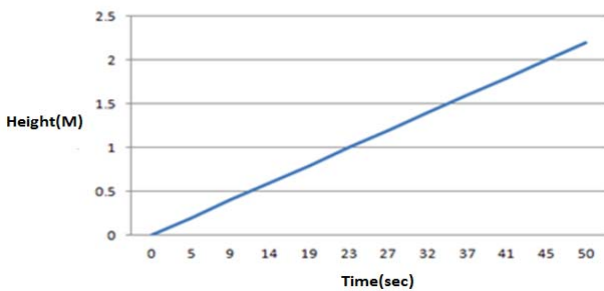
Figure 18: The relationship between sail lifting time and sail height in the eco-environmental leisure boat
