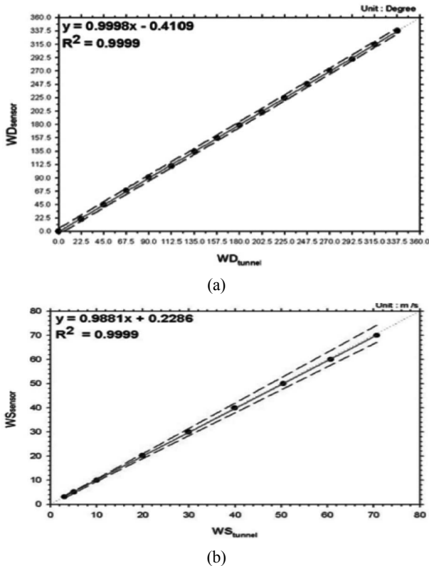
Figure 14: The graph showing the state of sensitivity of wind direction(a), wind speed(b)
