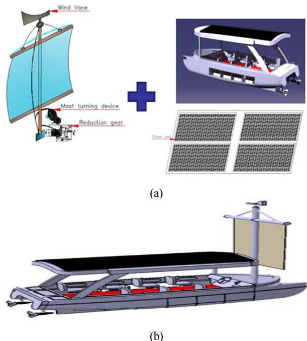
Figure 2: Schematic diagram showing a photovoltaic hybrid generating system (wind + solar energy)(a), eco-environmental leisure boat with same system(b)
