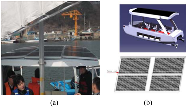
Figure 6: Actual image to show the photovoltaic panels used for photovoltaic generating system (a), its schematic assembled modelling image (b)
