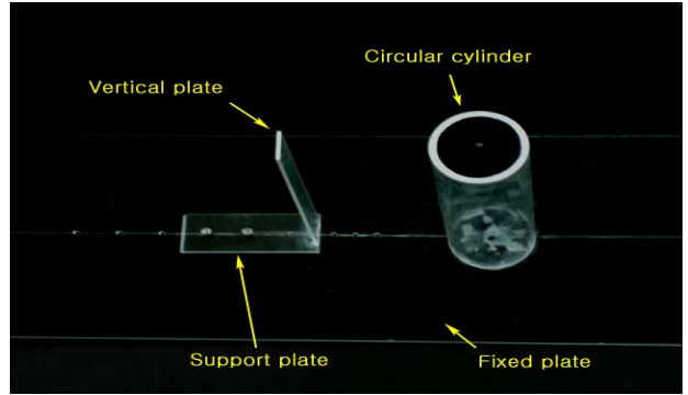
Figure 3: Photograph of experimental device
