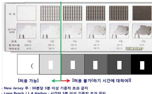
Figure 2: Ringelmann chart
