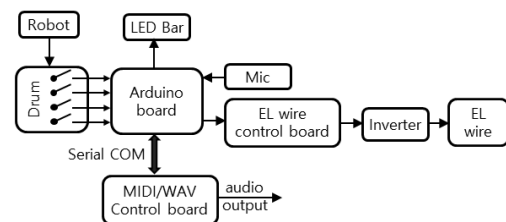
Fig. 6. Configuration of electronic drum
