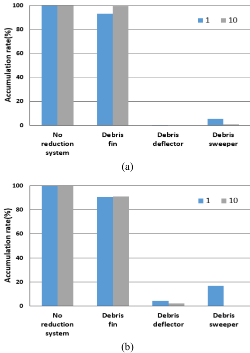
Fig. 8. Experimental result on debris reduction system (a) soft type (b) hard type
