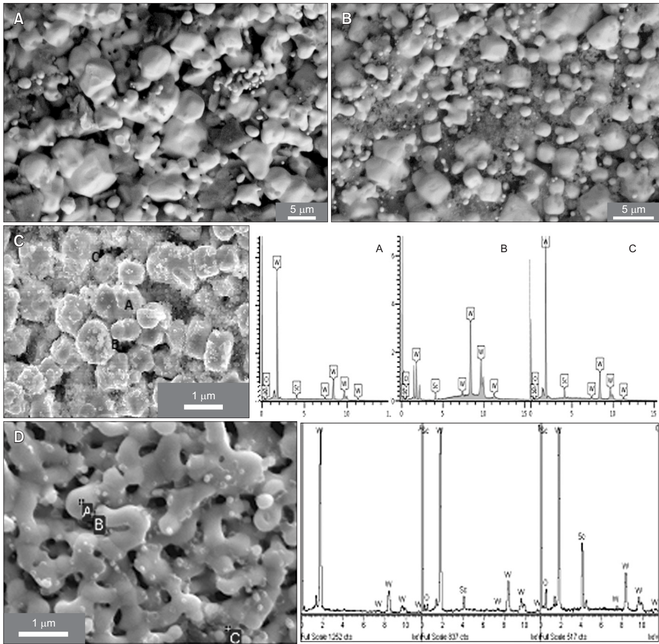
Fig. 1. Scanning electron microscope images of Sc 2 O 3 -W matrices prepared with Scandia doped tungsten powder obtained by mechanical mixing (A), liquid-solid doping (B), and Sol-Gel method and EDS result (C), Re-Sc 2 O 3 -W cathode prepared by liquid-solid doping and EDS result (D).
