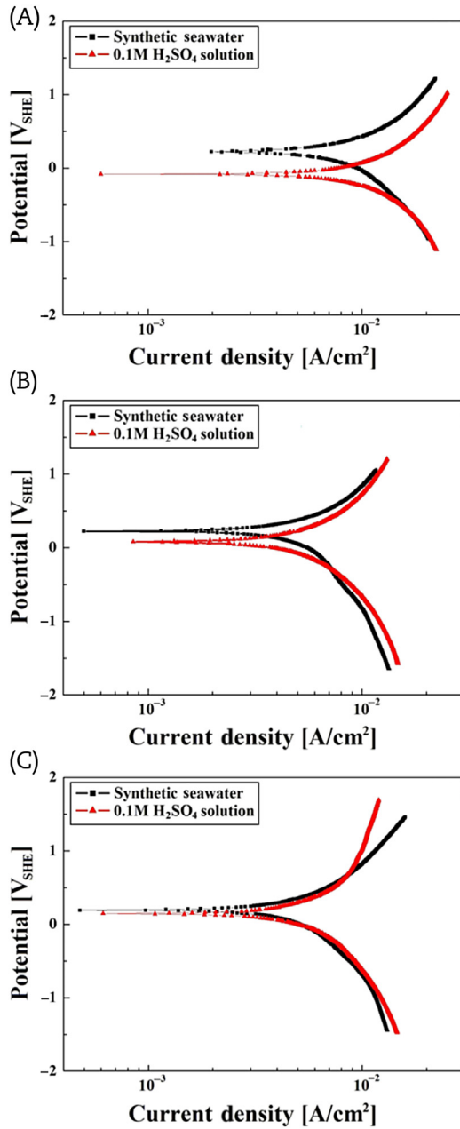
Fig. 3 – Typical polarization curves of 0.087% Gd-lean duplex stainless steels in an artificial sea water and 0.1 M H 2 SO 4 solution at 25°C with cold rolling directions. Surface normal to (A) rolling direction (RD), (B) transverse direction (TD), and (C) short transverse (ST) direction.
