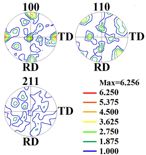
Fig. 2 – Typical crystallographic texture of 100, 110, and 211 poles.
