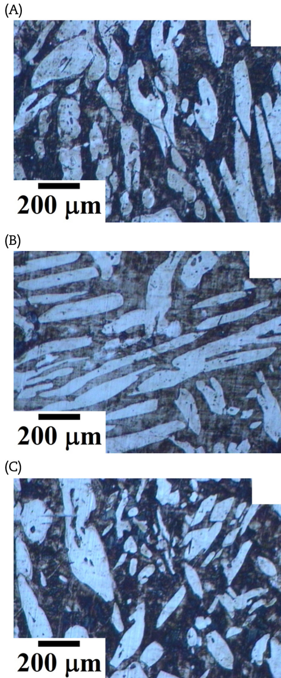
Fig. 1 – Microstructure of the 0.087% Gd lean duplex stainless steel with cold rolling directions: surface normal to (A) short transverse (ST) direction, (B) transverse direction (TD), and (C) rolling direction (RD).
