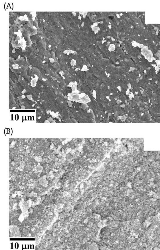
Fig. 4 – Typical scanning electron microscopy images of the worn surfaces. (A) Air and (B) artificial seawater.
