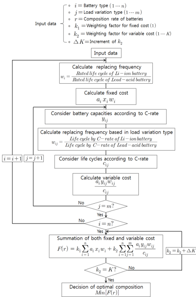
Fig. 4. Flowchart calculating optimal composition rate.
