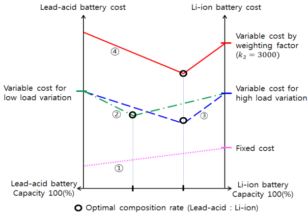
Fig. 3. Concept of optimal composition rate.
