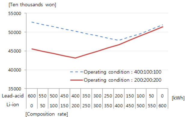
Fig. 7. Optimal composition rate for increasing high variation load.
