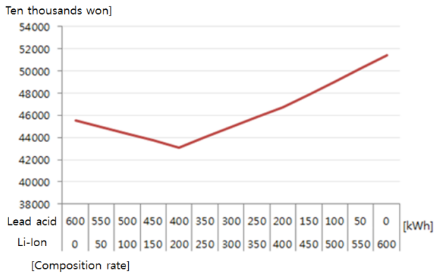
Fig. 5. Optimal composition rate according to economic mechanism by load characteristic
