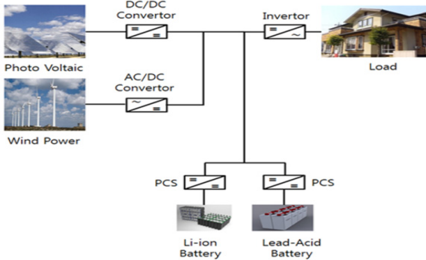
Fig. 2. Hybrid ESS installed in off-grid.
