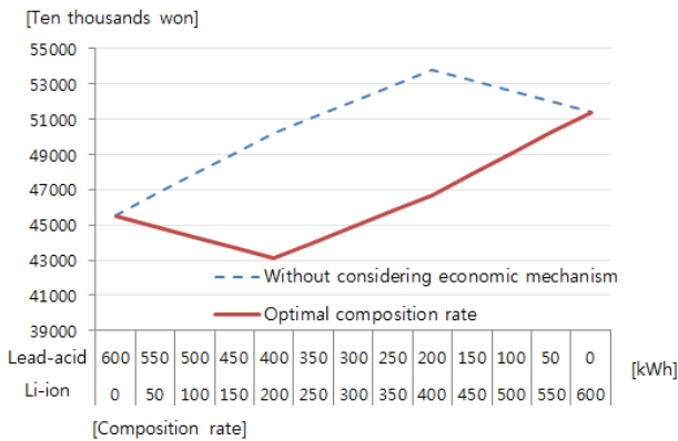
Fig. 6. Optimal composition rate according to economic mechanism by discharging characteristic of each battery
