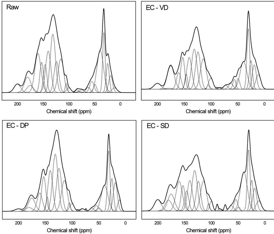
Fig. 3. The fitted 13 C NMR spectra of raw and ash-free coal samples.
