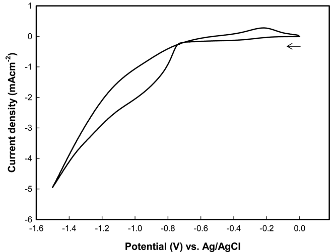
Fig. 1. CV curve of Ti-mesh in 0.1 M \text{Co}(\text{NO}_3)_2 \cdot \text{H}_2\text{O} solution at 0.5 \text{ mV s}^{-1} scan rate.
