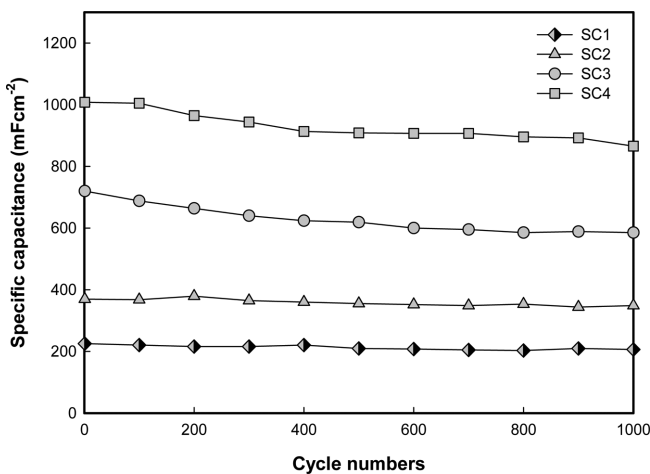
Fig. 7. Cycling performance of SC1, SC2, SC3, and SC4 electrodes in 1 M KOH electrolyte at 8 mA cm -2 .
