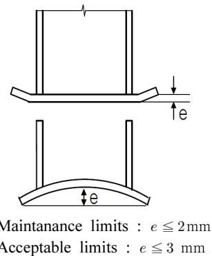
Fig. 2. The limits of deformation (Base plate)
