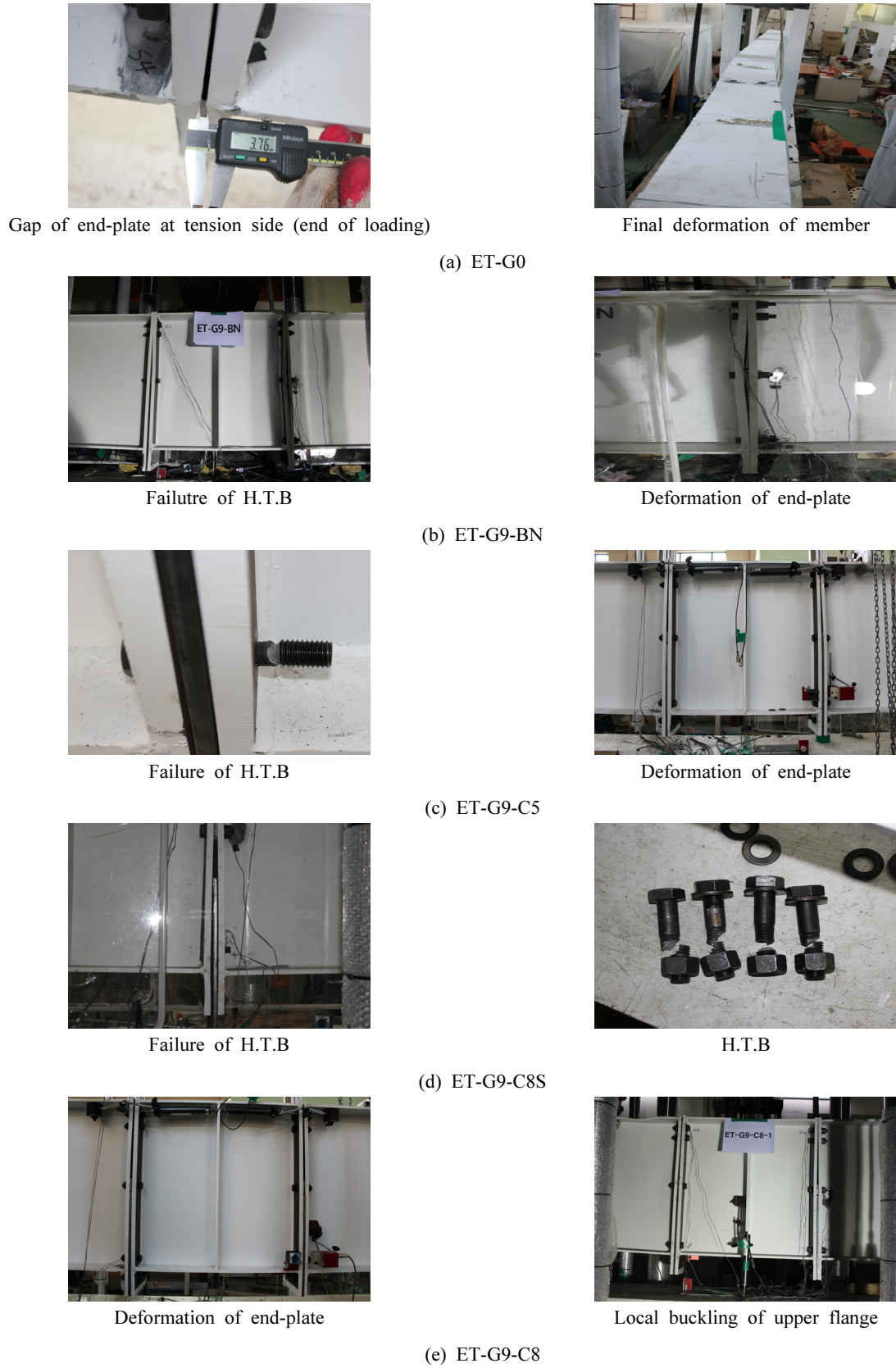
Fig. 12. Failure mode of specimens
