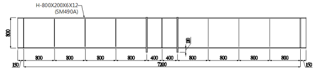
Fig. 4. Specimen type
