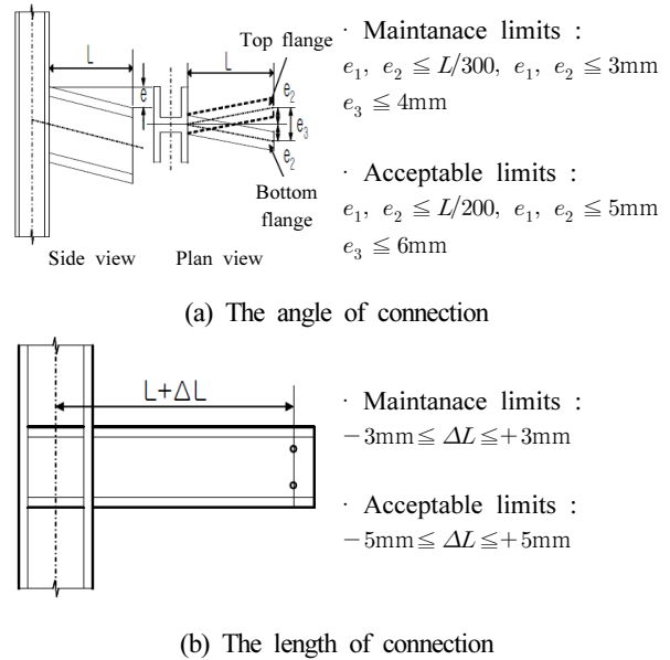
Fig. 1. The limits of deformation (connection)
