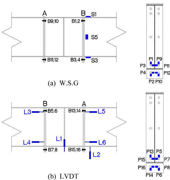
Fig. 9. Location of L.V.D.T and W.S.G
