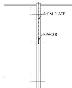
Fig. 6. Gap inducing
