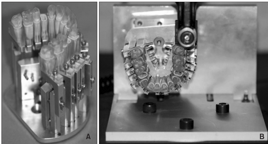
Figure 1. The stereolithographically-made typodont system. A , The maxillary teeth were aligned to their ideal positions according to a Broad Arch Form (Ormco). For the evaluation of frictional force in sliding mechanics during extraction space closure, the maxillary first premolar was removed from the typodont. B , The stereolithographically-made typodont system and testing apparatus.
