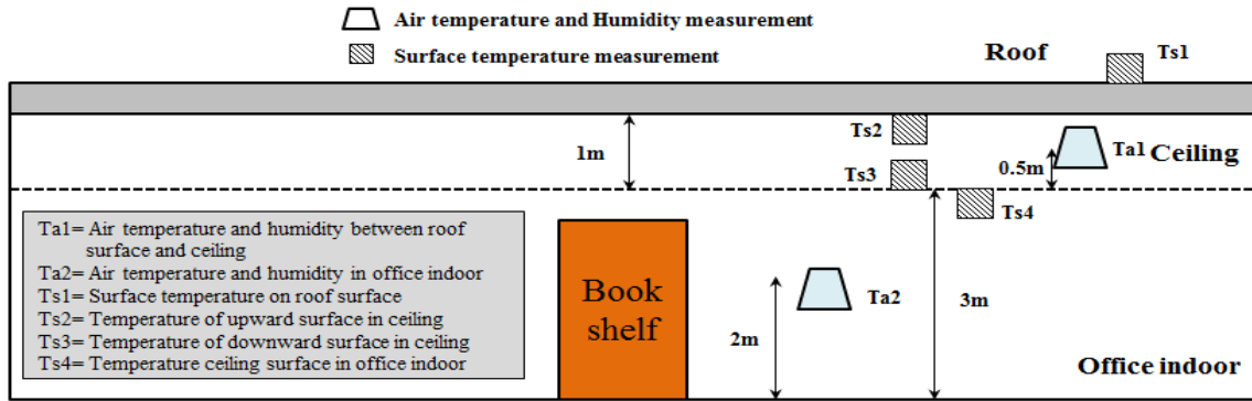
Fig. 4. Position of measurement equipment in office indoor
