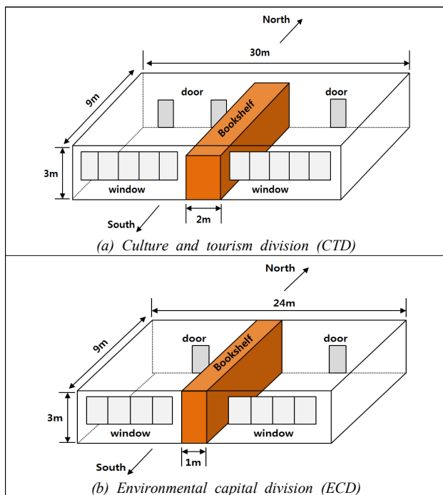
Fig. 2. Layouts and structures of two office rooms
