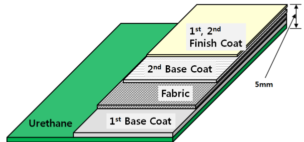
Fig. 3. Cross section of constructed Cool roof
