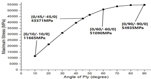
Fig. 4. Graph of maximum equivalent stress due to stacking angle of unidirectional CFRP
