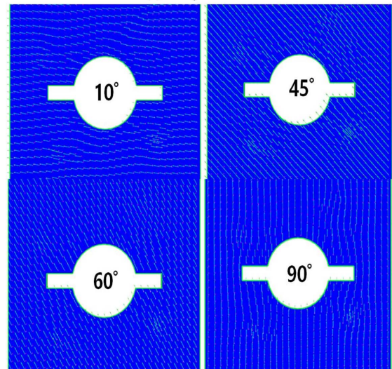
(b) Stacking angle of unidirectional carbon fiber
