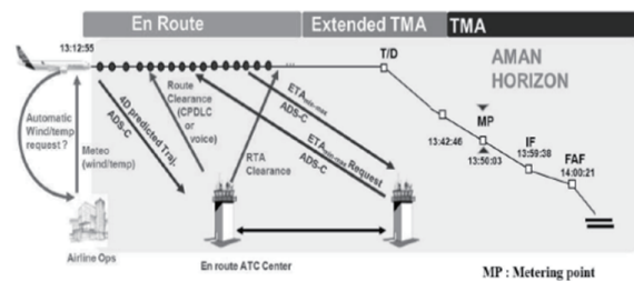
Fig. 2. Summary of TBO procedure. [16]
