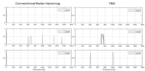
Fig. 7. Total loss of separation with CIP
