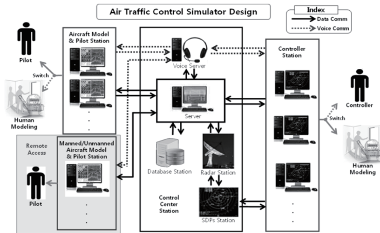
Fig. 3. Air Traffic Control Simulator Structure.
