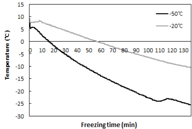
Fig. 1. Change in temperature of dried persimmons during freezing at different temperatures.
