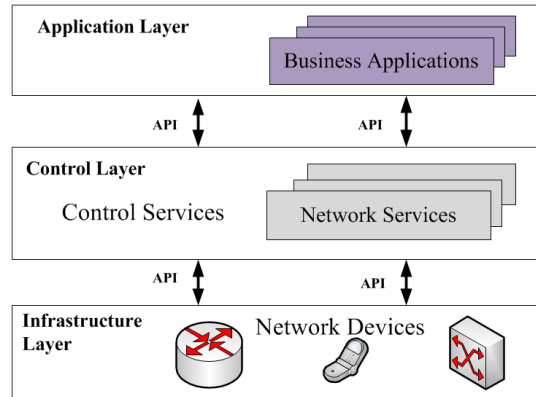
Fig. 1. Architecture of Software Defined Networking.
