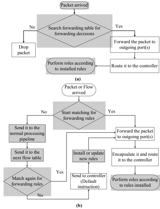
Fig. 2. Algorithm for (a) Conventional IP-based Network (b) Proposed Software Defined Networking
