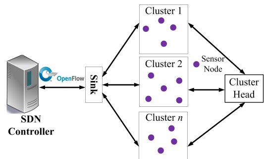
Fig. 5. Proposed SD-ISN Scenario for Simulation.
