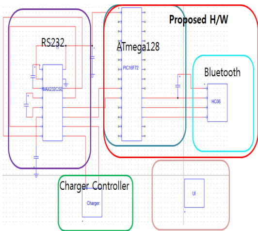
Fig. 9. Proposed H/W Schematic
