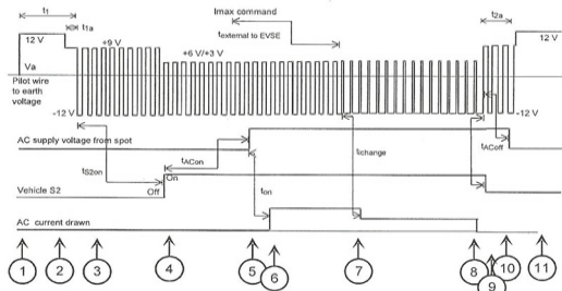
Fig. 4. Charging cycles[4]
