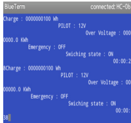
Fig. 11. Proposed Low Cost Charger UI
