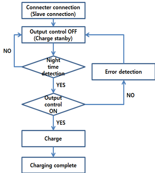
Fig. 6. Midnight charging algorithm
