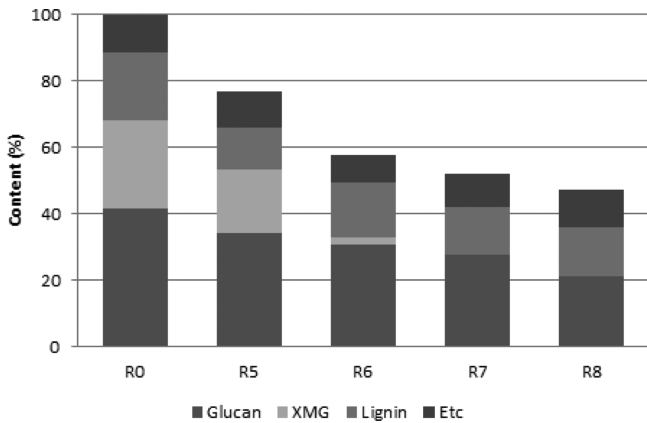
Fig. 5. Component contents of pretreated rigida on various conditions (R5, R6 used an ethanol and surfuric acid as an organosolv, respectively. R7, R8 are the 2-stage flow-through pretreatment).
