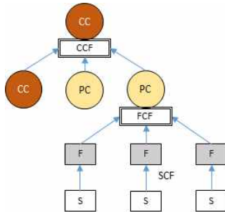
Fig. 2. Context Relation Diagram
