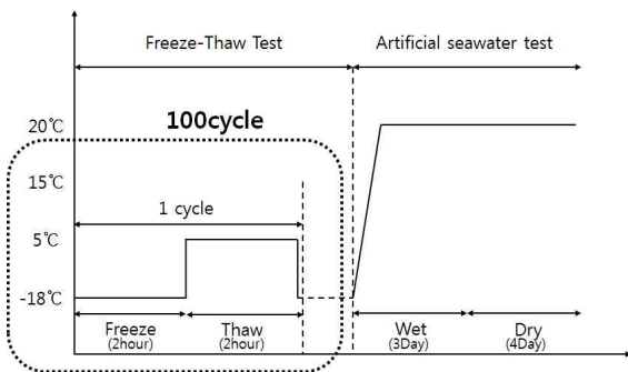
Fig. 3. Planned Freeze-thaw cycles of accelerated test (case 2, 100 cycle).
