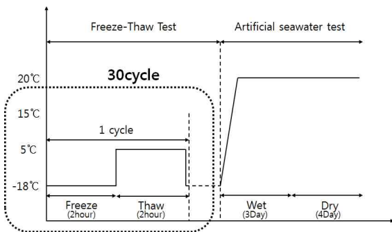
Fig. 2. Planned Freeze-thaw cycles of accelerated test (case 1, 30 cycle).
