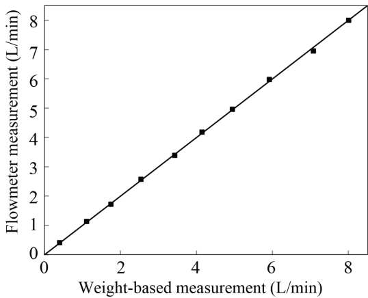
Fig. 7 Comparison of the measurement of the flow rates using the flowmeter with the weight-based measurements
