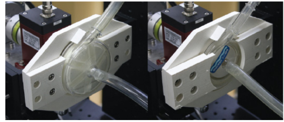
Fig. 3 Supporting plates and magnetic couplings constructed by 3D printing for commercial blood pump A (left) and B (right)
