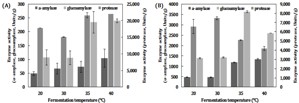
Fig. 2. Effects of enzyme activity on various fermentation temperature of solid starter.
