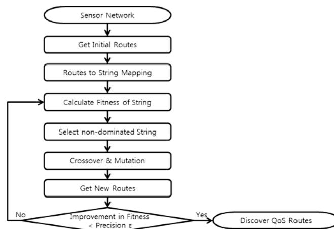
Fig. 3. Near-optimal QoS-routing algorithm
