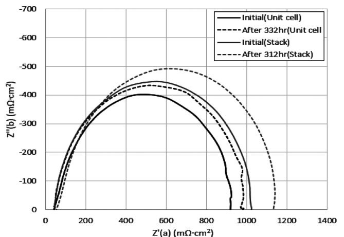
Fig. 6. Comparison of impedance between unit cell and stack after accelerated degradation test of electrolyte membrane.
