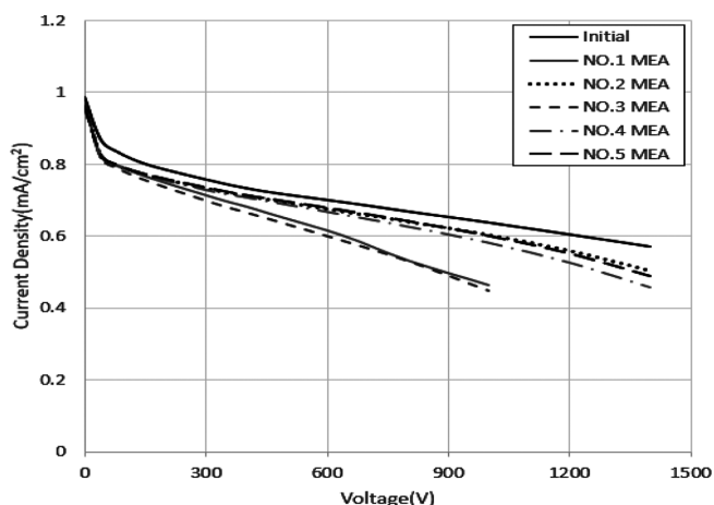
Fig. 1. I-V curves of MEAs in 5 cell stack after accelerated degradation test of electrolyte membrane for 312 hours.
