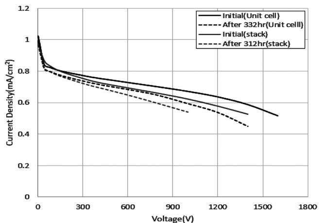
Fig. 5. Comparison of I-V performance between unit cell and stack after accelerated degradation test of electrolyte membrane.
