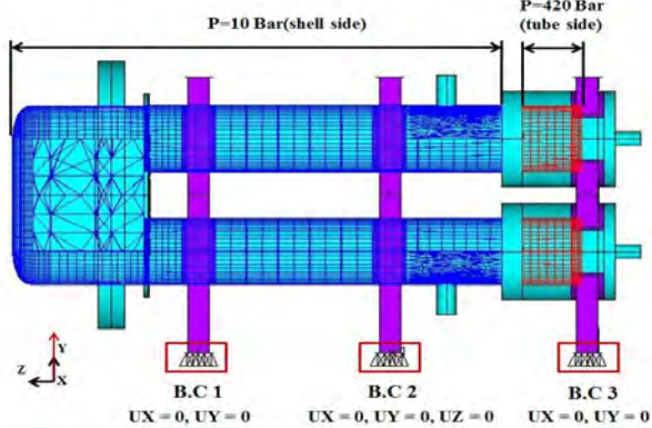
Figure 5: Boundary and pressure condition of the vaporizer
