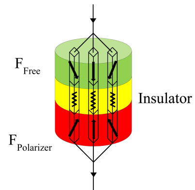
Fig. 3. (Color online) Schematic diagram of parallel resistance model for MTJ. Each cell of MTJ is connect by parallel, and the tunneling between polarizer and free layer are modeled a resistance, whose value is a function of the angle between spins.
