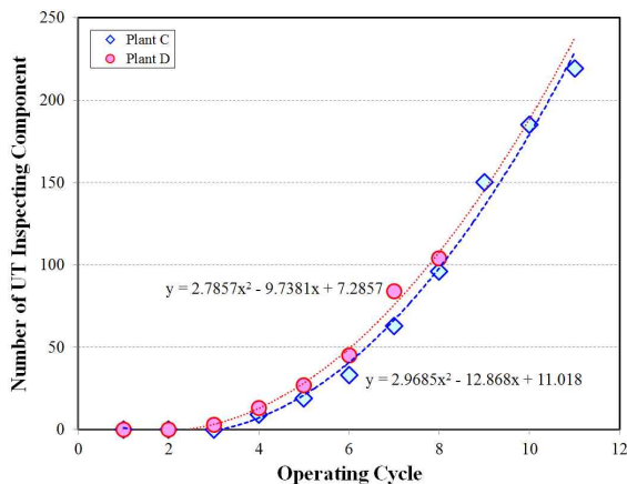
Fig. 4. Distribution chart of inspected components over three times of two operating plants.
