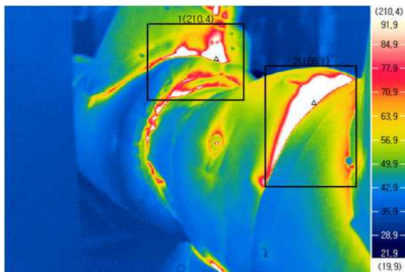
Fig. 2. Thermal imageries of piping with removable insulation.
