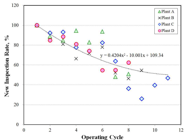
Fig. 3. New inspection rate for a total inspecting number by cycle.
