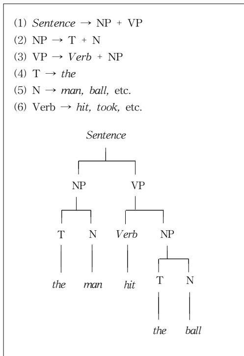
Fig. 1. Examples of Phrase Structure Grammar / Constituency Structure (cited from [13])
