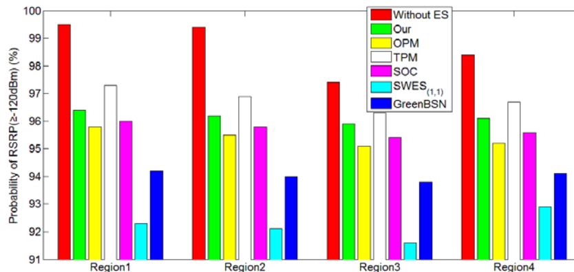
Fig. 11. Probability of RSRP of four regions
