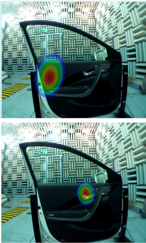
Fig. 8 Results of sound field visualization of door latch operating moment
