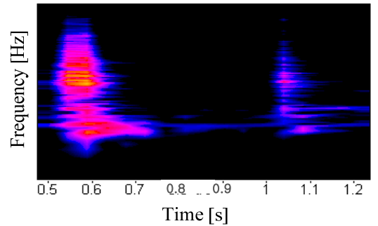
Fig. 3 Time-frequency property of 'Unlocking' sound
