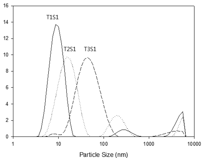
Fig. 3. Particle size distributions of TiO 2 -SnO 2 sols prepared with different SnCl 4 ·5H 2 O content at 60 °C.
