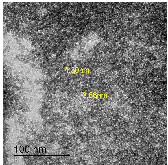
Fig. 2. TEM image of TiO 2 -SnO 2 nanoparticles prepared at 60 °C.
