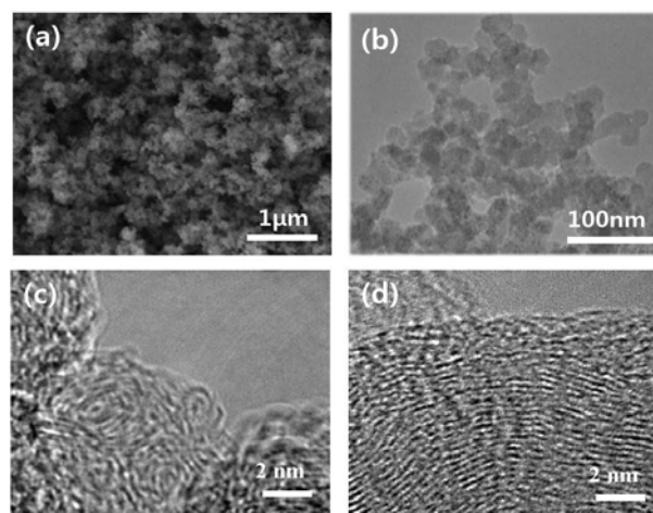
Figure 2: FESEM image of raw CNB (a), TEM image of raw CNB (b), HRTEM image annealed at 550 °C(c), and HRTEM image annealed at 850 °C (d)
