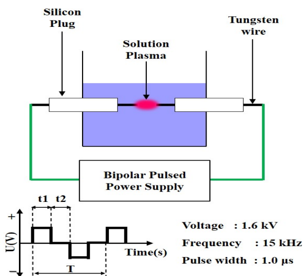
Figure 1: Schematic of solution plasma process
