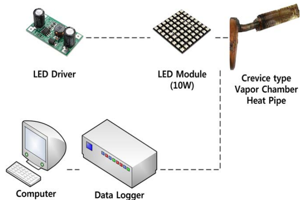
Figure 2: Schematic diagram of an experimental set up
