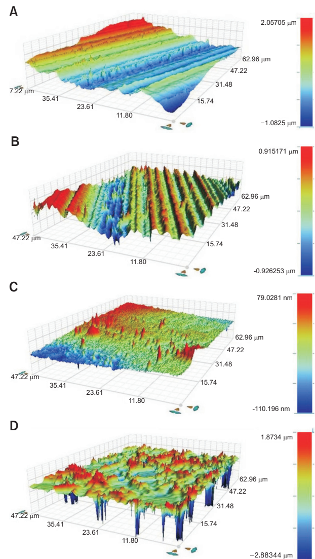
Figure 4. Three-dimensional optical profiler images of zirconia surface (magnification \times 100 ). A, Nonglazed zirconia; B, nonglazed zirconia + sandblasting; C, glazed zirconia; and D, glazed zirconia + sandblasting and acid etching. The right side of each figure includes a colorimeter band representing the height of each spot as different color.
