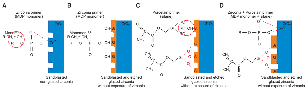
Figure 6. Chemical interaction models between primer and various zirconia surfaces. A, Nonglazed zirconia with zirconia primer; B, glazed and roughened zirconia with zirconia primer, showing mismatched interaction between zirconia primer (MDP) and the glazed surface; C, glazed and roughened zirconia with porcelain primer; and D, glazed and roughened zirconia with both primers.
