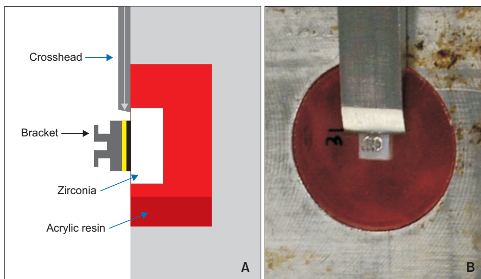
Figure 1. A, Schematic illustration of the shear-bond-strength test. B, Equipment for measuring shear bond strength.
