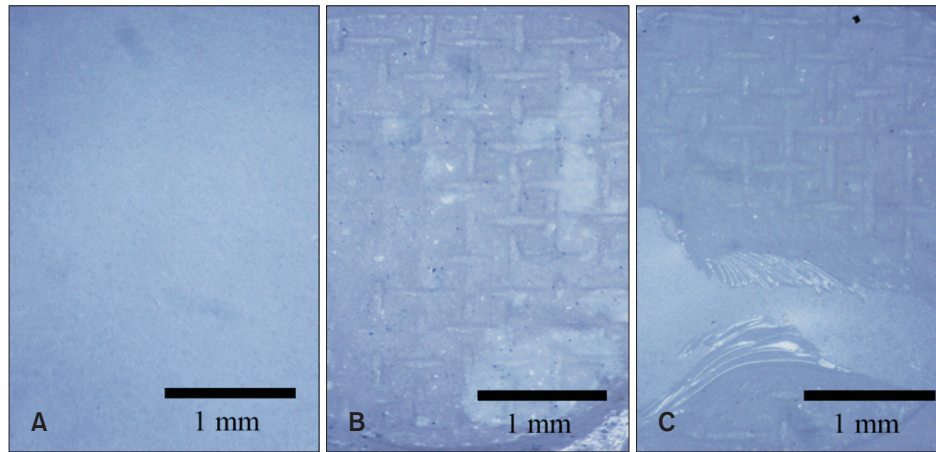
Figure 5. Stereoscopic micrographs of debonded surfaces (magnification \times 16 ). A, Adhesive failure between zirconia and resin cement; B, adhesive failure between resin cement and bracket base; C, complex adhesive and cohesive failure.
