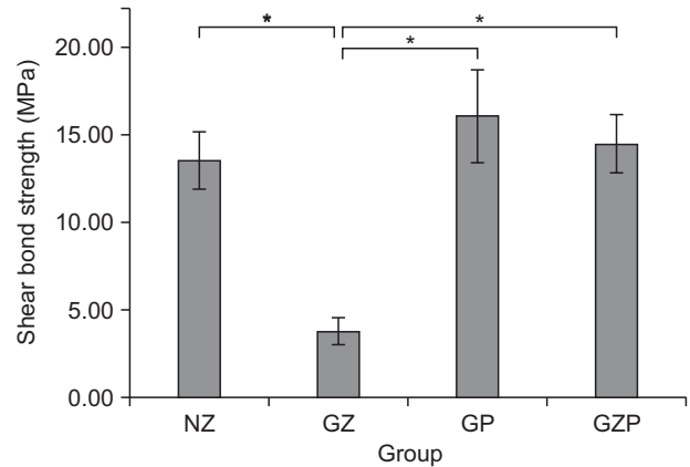
Figure 2. Comparison of the values of shear bond strength. *Statistically significant ( p < 0.05 ).
