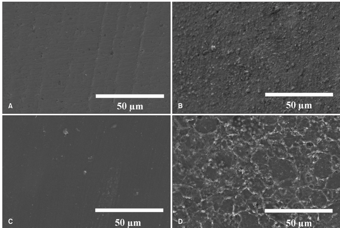
Figure 3. Scanning electron microscopy images of zirconia surface (magnification \times 1,000 ). A, Nonglazed zirconia; B, nonglazed zirconia + sandblasting; C, glazed zirconia; and D, glazed zirconia + sandblasting and acid etching.
