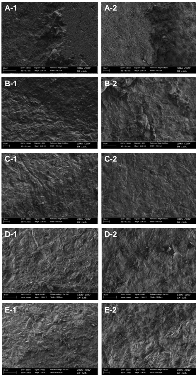
Fig. 6. Scanning electron microscope image of zirconia surface after shear-bond strength test ( \times 2,000 magnification, -1: before thermocycling, -2: after thermocycling). (A) P: Permaceem 2.0, (B) C: Clearfil™ SA Luting, (C) M: Multilink® Speed, (D) R: RelyX™ U200, (E) G: G-Cem LinkAce™.
