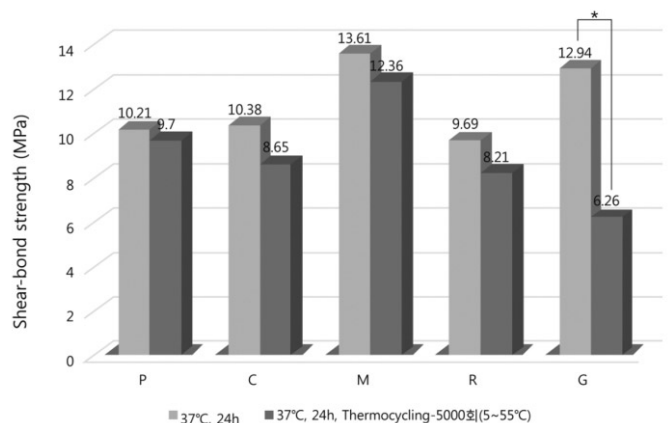
Fig. 3. Mean shear bond strength (*: Statistically significant with P<.05).
