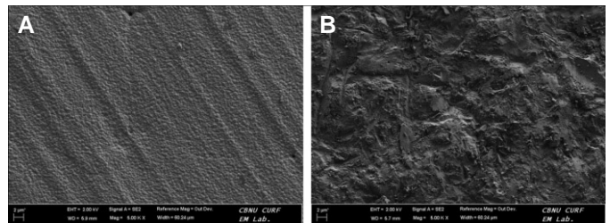
Fig. 5. Scanning electron microscope image of zirconia surface ( \times 5,000 magnification). (A) polished with 1 \mu\text{m} diamond paste, (B) sandblasting with 50 \mu\text{m} \text{Al}_2\text{O}_3 .
